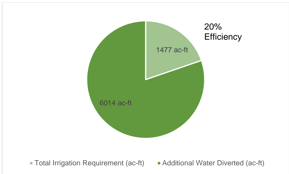
Figure 2.6.1.2. Calculated System Efficiency of the Short Ditch
